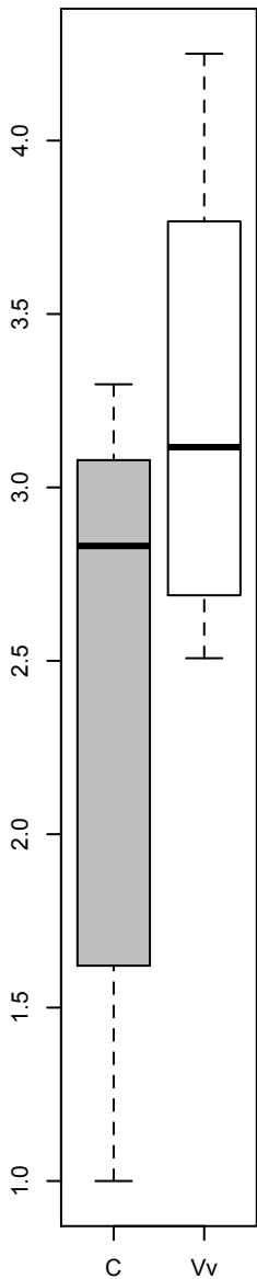
Cg-Sptlc1
